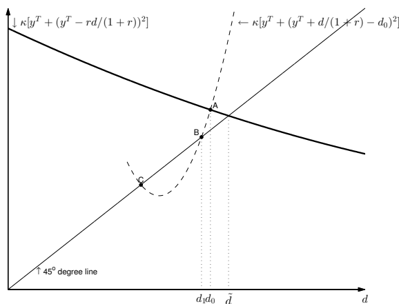
Figure 2: Multiple Equilibria With Flow Collateral Constraints
