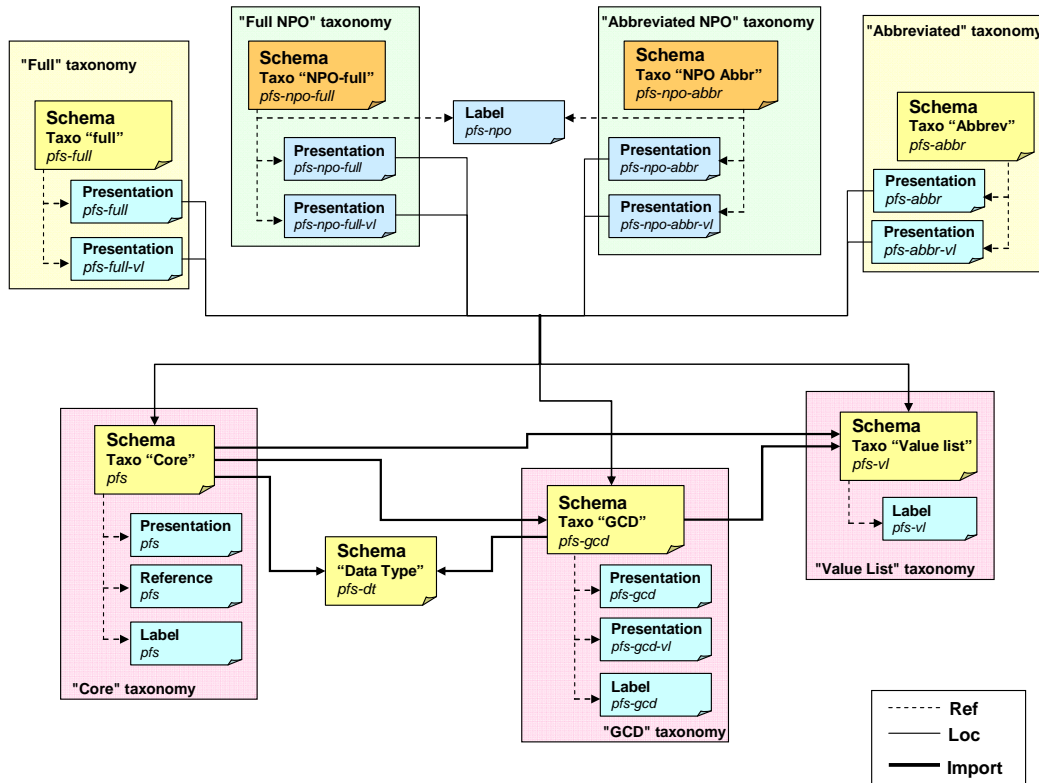
Figure 2: Taxonomy architecture - be-fr-pfs-ci-2011-04-01
